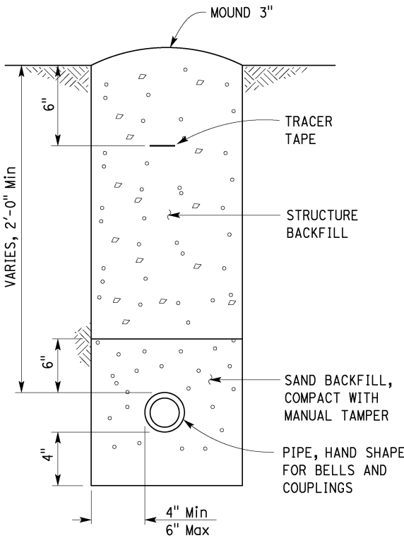
3 SEWER / FORCE MAIN NO SCALE
