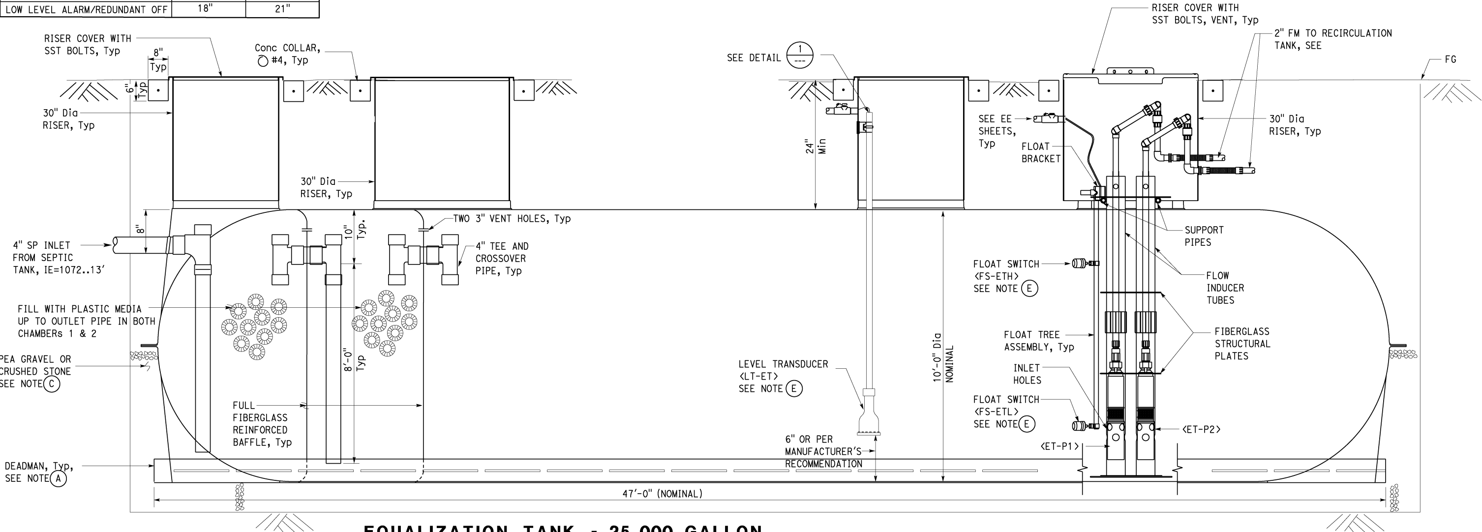
EQUALIZATION TANK - 25,000 GALLON NO SCALE
