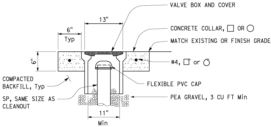
A COTG IN VALVE BOX NO SCALE
